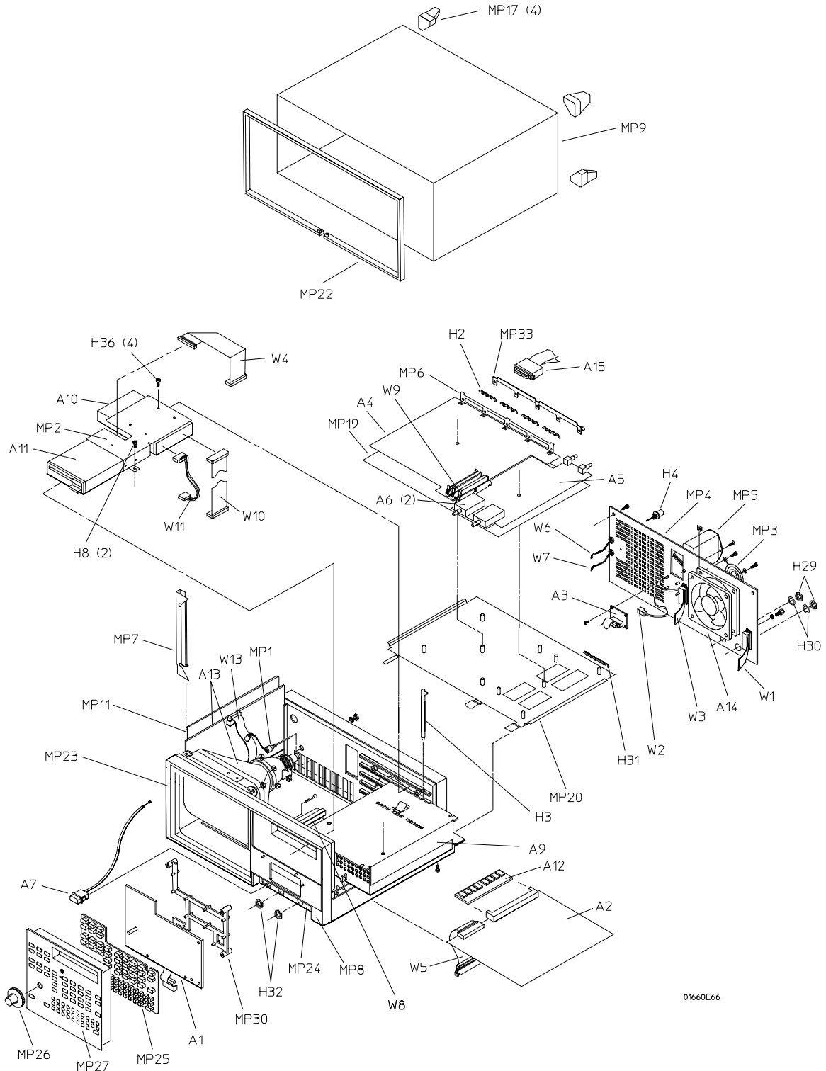
HP 166xCS Logic Analyzer Exploded View
